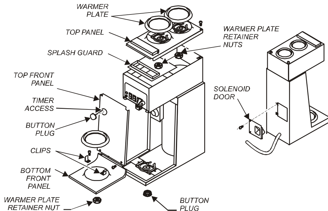
Fig. 9 Access Panels
