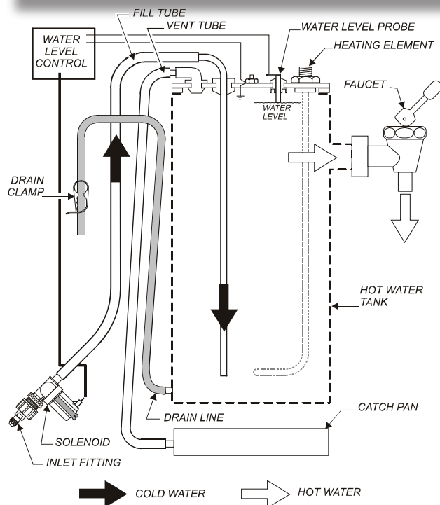
Fig. 3 Dispenser Operation Diagram
