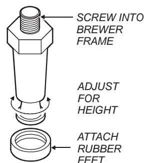
Fig. 2 Adjustable Legs
