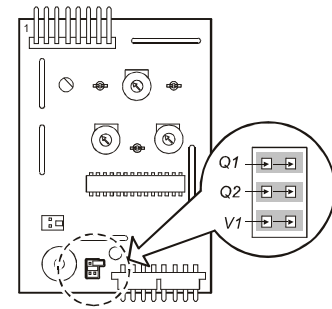
Fig. 19 Controller Jumpers
