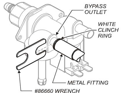
P/N 86660 Braided Hose Wrench
