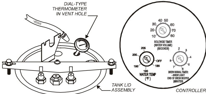
Fig. 14 Checking and Adjusting Brew Temperature
