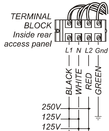
Fig. 3 Electrical Installation
