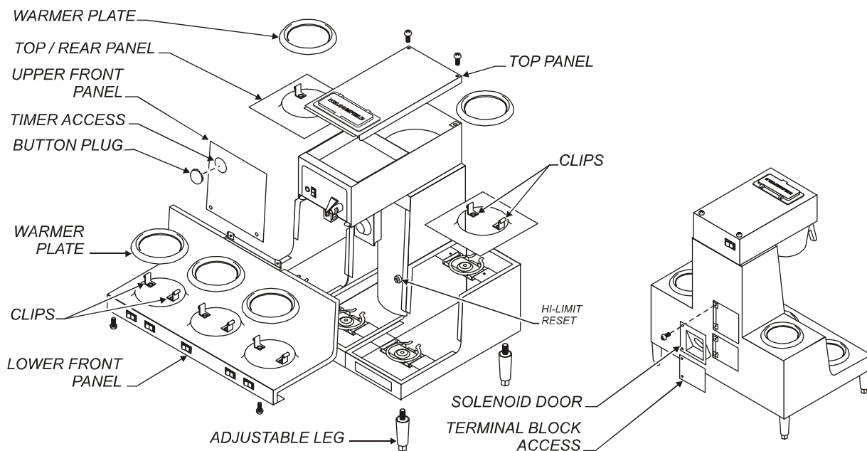
Fig. 9 Access Panels
