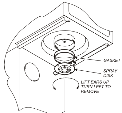
Fig. 8 Cleaning
