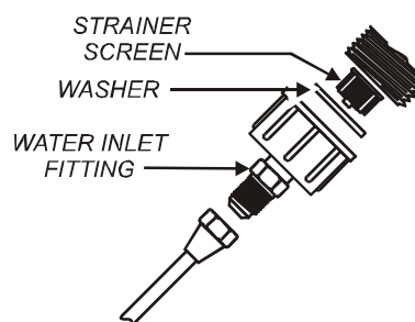
Fig. 14 Clean Strainer Screen
