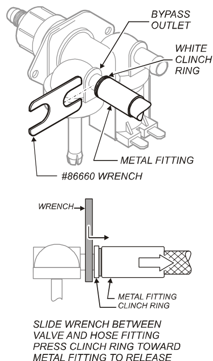
Fig. 13 Remove Faucet Supply from Solenoid
