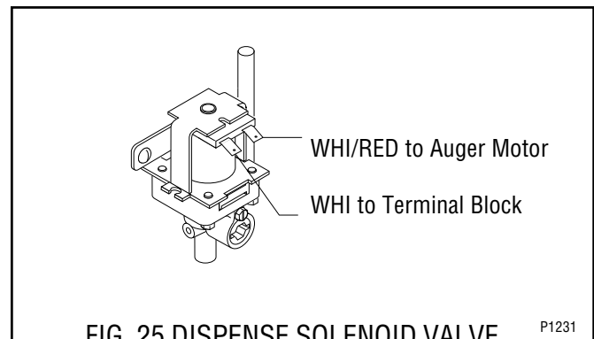
FIG. 25 DISPENSE SOLENOID VALVE TERMINALS
