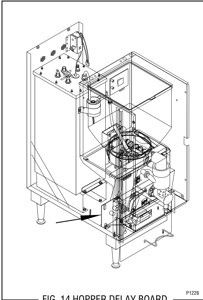
FIG. 14 HOPPER DELAY BOARD
