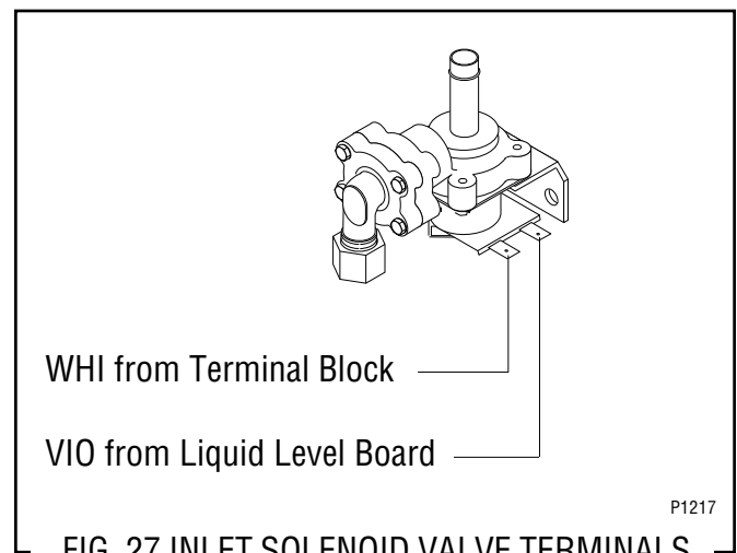
FIG. 27 INLET SOLENOID VALVE TERMINALS
