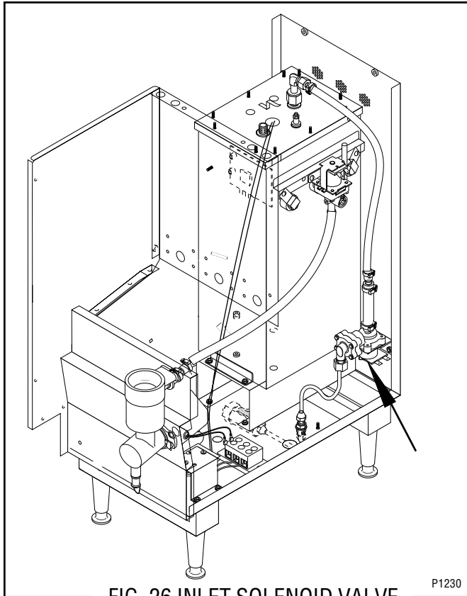
FIG. 26 INLET SOLENOID VALVE
