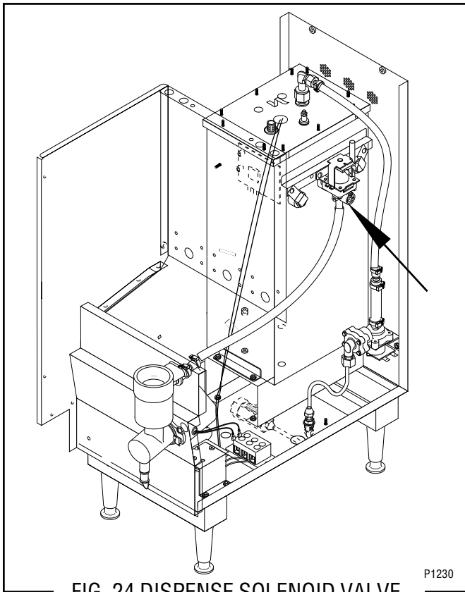
FIG. 24 DISPENSE SOLENOID VALVE
