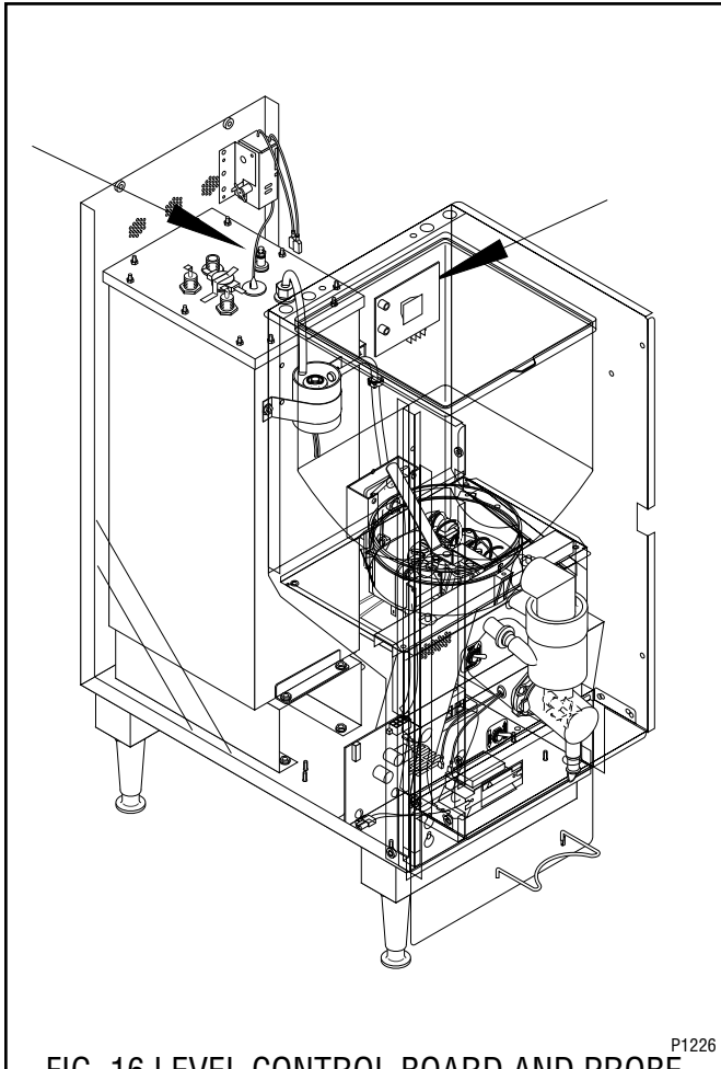
FIG. 16 LEVEL CONTROL BOARD AND PROBE
