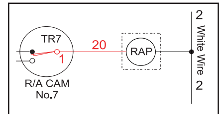
Rinse-aid dispensing pump & cycle timer cam No.7 with timer microswitch
