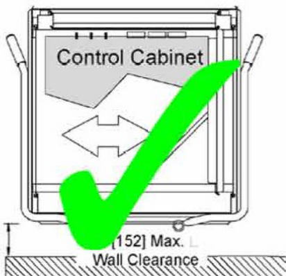
Straight-through Configuration
