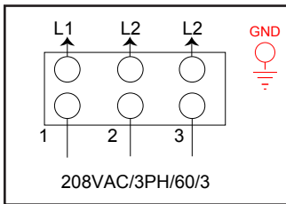
Main terminal block and ground lug
