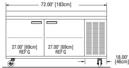
Elevation View 18672BSTM
