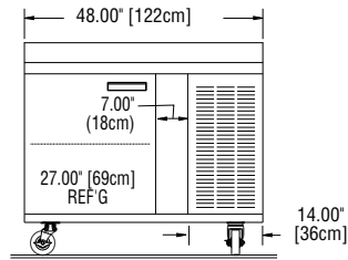
Elevation View 18648BSTM
