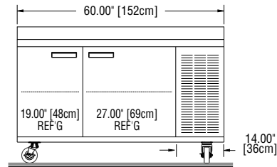
Elevation View 18660BSTM
