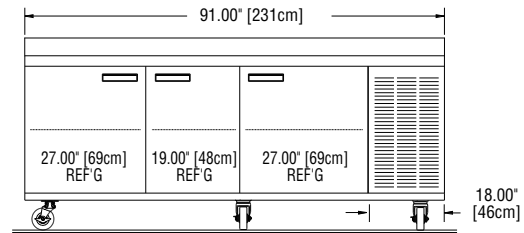
Elevation View 18691BSTM
