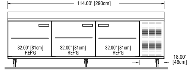
Elevation View 186114BSTM
