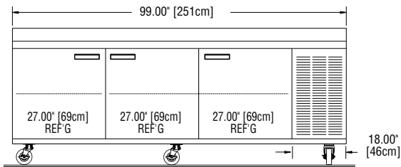
Elevation View 18699BSTM
