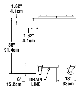
END VIEW ALL MODELS
