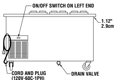
ELEVATION VIEW KCF-60
