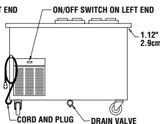
ELEVATION VIEW KCF-50
