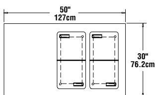
PLAN VIEW KCF-50
