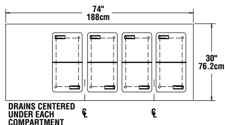
PLAN VIEW KCM-74
