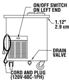
ELEVATION VIEW KCM-36
