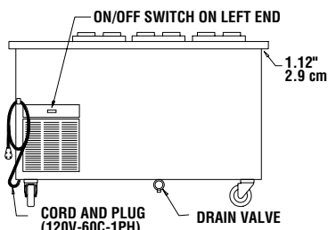
ELEVATION VIEW KCM-60
