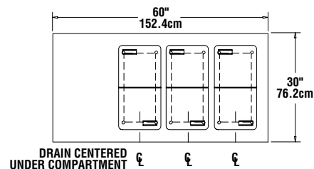
PLAN VIEW KCM-60
