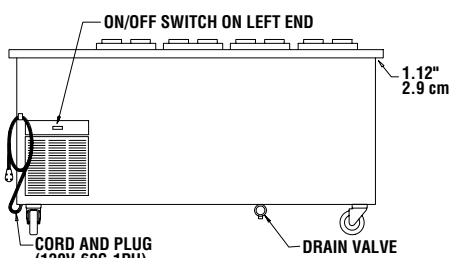
ELEVATION VIEW KCM-74
