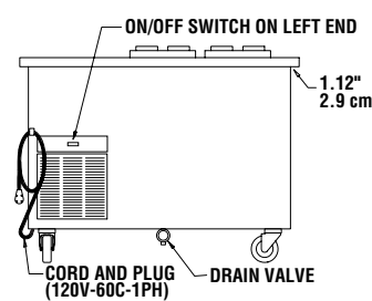
ELEVATION VIEW KCM-50
