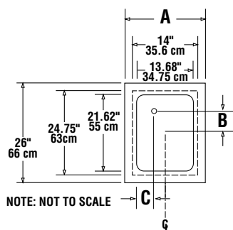
PLAN VIEW MODEL N8018
