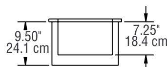
TYPICAL END VIEW
