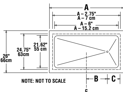
TYPICAL PLAN VIEW N8000 MODELS (EXCEPT N8018)
