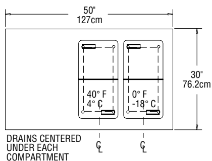
PLAN VIEW SCFM-50
