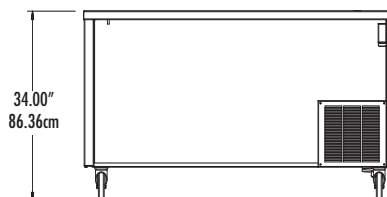
Elevation View SPF-66
