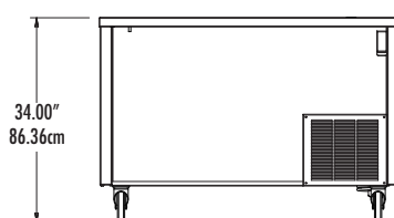
Elevation View SPF-52
