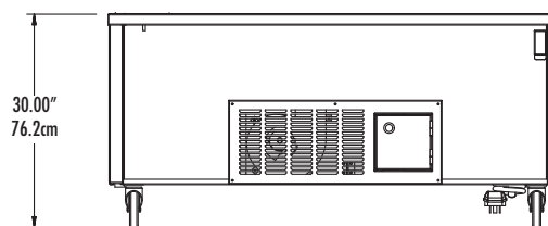
Elevation View SPH-64EW
