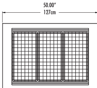
Basket Detail
