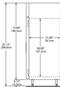
END VIEW ALL SECTION UNITS
