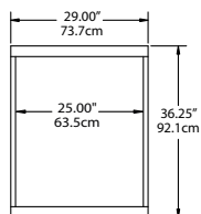
PLAN VIEW SSHPT1-S, SAHPT1-S, SMHPT1-S SSHPT1-SH, SAHPT1-SH, SMHPT1-SH
