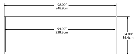
PLAN VIEW SSRI3-S, SARRI3-S, SMRI3-S
