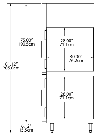
END VIEW
