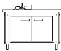
DCHS-51 Elevation View
