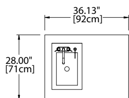
DCHS-DI Plan View
