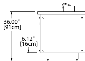
DCHS-51 Right Side View
