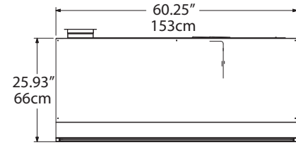
Plan View, ASM-60
