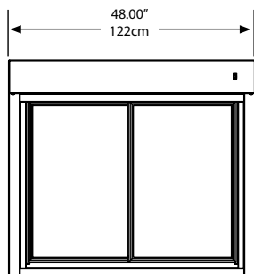
Elevation View F5PR48N
