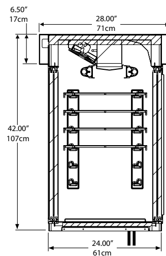
Right End View F5PR48N, F5PR72N
