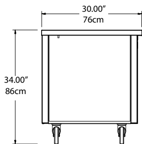
Elevation View SPCS-30W
