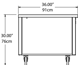
Elevation View SPCS-36EW
