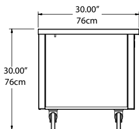
Elevation View SPCS-30EW
