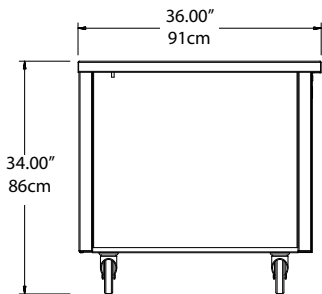
Elevation View SPCS-36W
