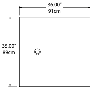
Plan View SPCS-36W, SPCS-36EW
