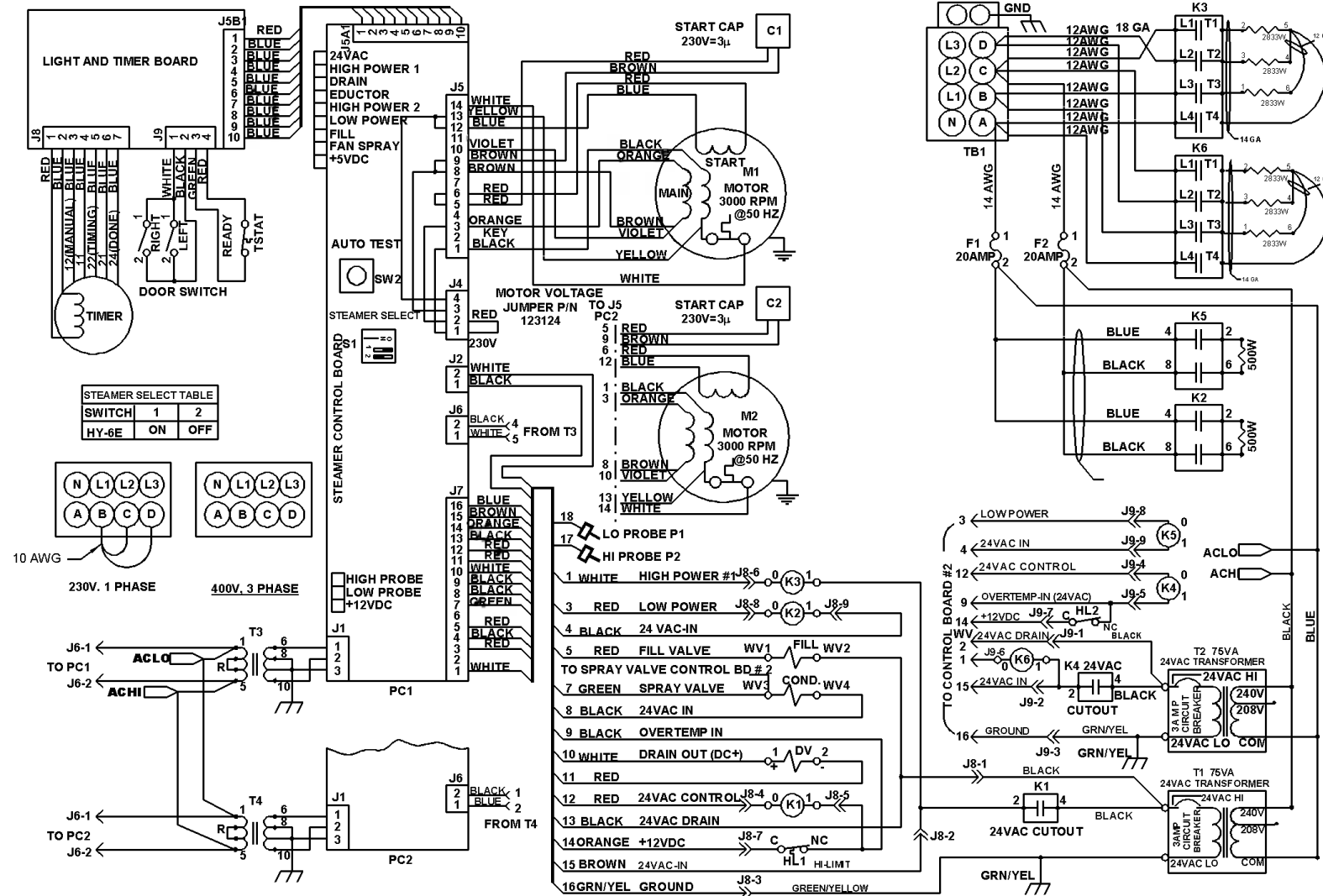
HY-6E (CE) WIRING DIAGRAM P/N 128699 REV A
