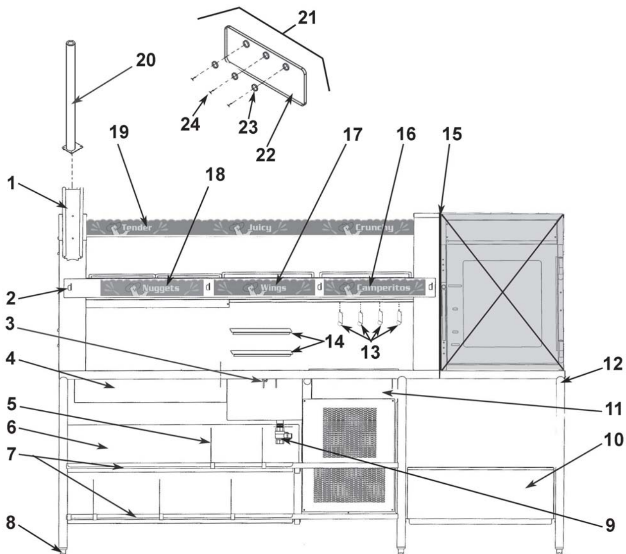
Figure 4-1. Customer Side Parts
