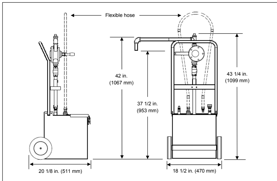
ODS-100 fryer oil disposal system
