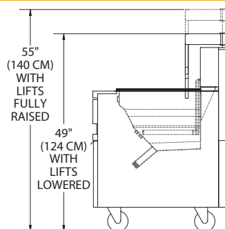
Side View With Lifts
