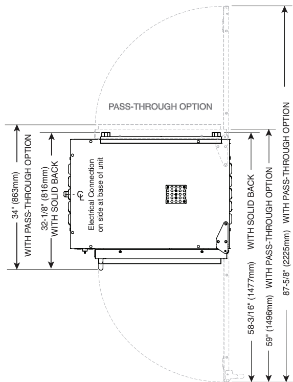
SINGLE PANE FLAT GLASS DOOR
