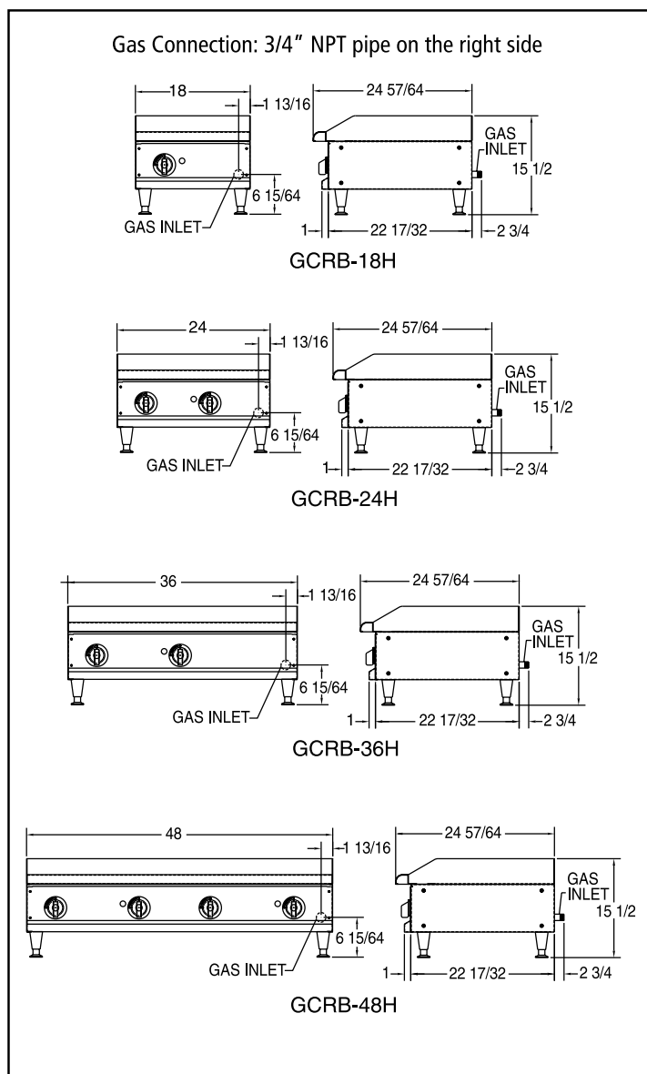
Model GCRB Gas CharRock Broiler
