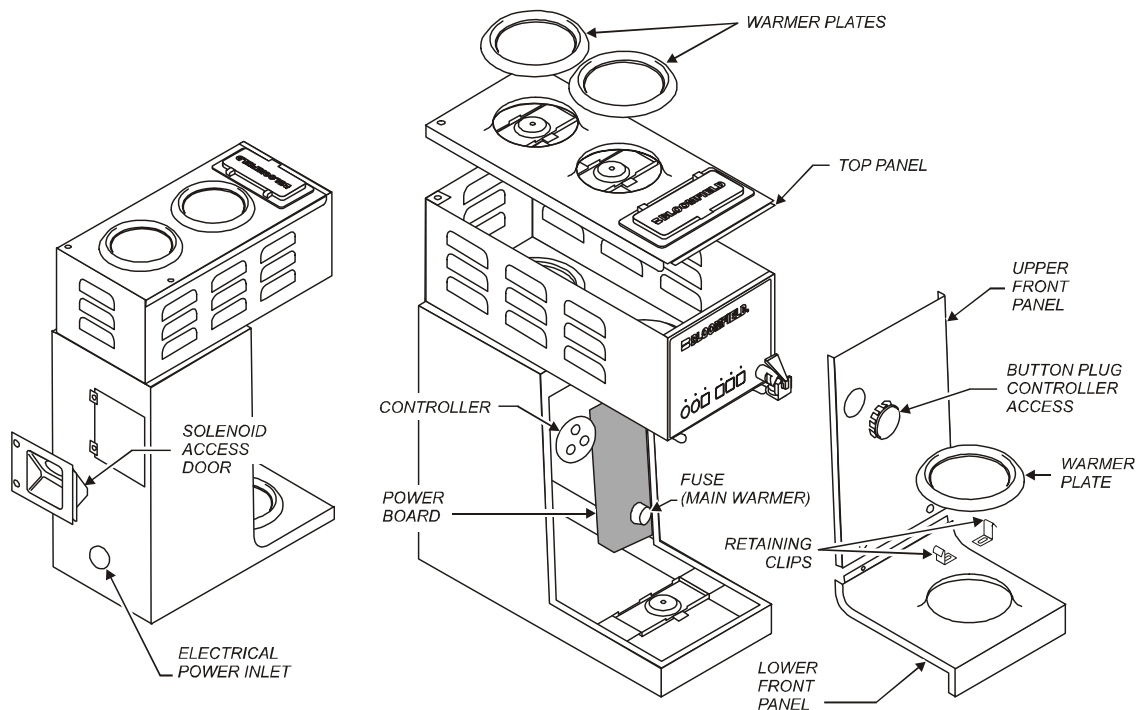
Fig. 12 Access Panels
