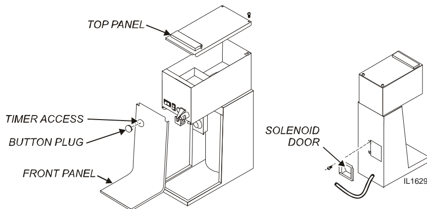
Fig. 9 Access Panels
