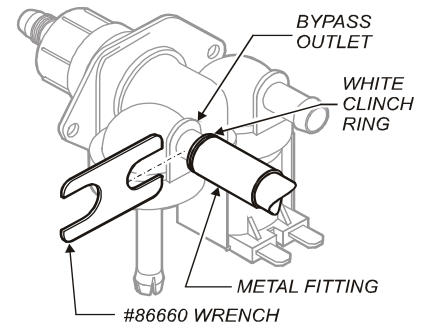
P/N 86660 Braided Hose Wrench
