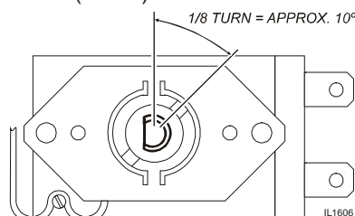
Fig. 11 Adjust Thermostat
