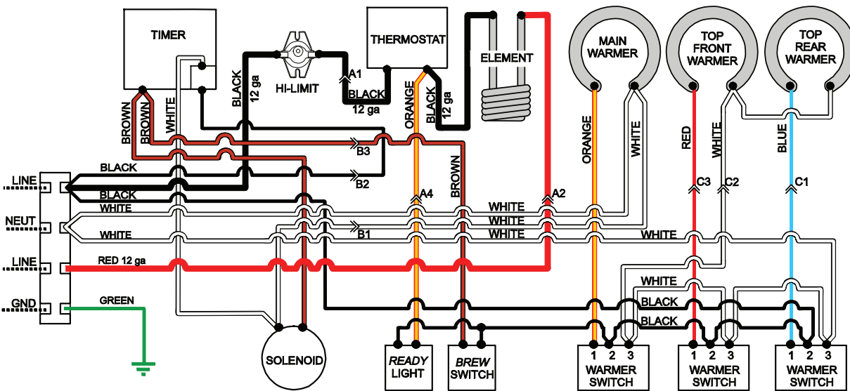
MODEL 9016 p/n 72356
