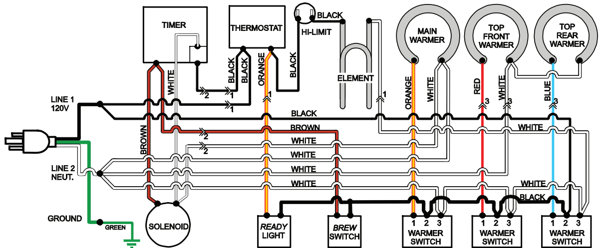
MODEL 9012 p/n 71725
