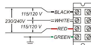
Fig. 3 115/240V Terminal Block
