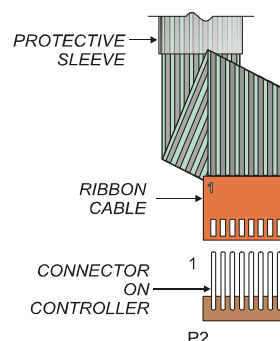
Fig. 19 Keypad Ribbon Cable Hook-Up
