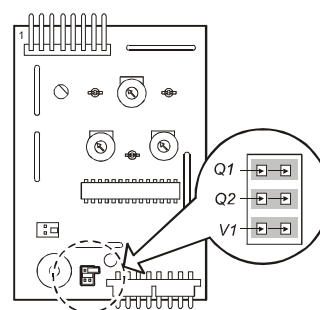
Fig. 18 Controller Jumpers
