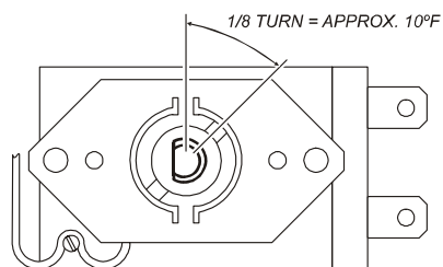
Fig. 10 Adjust Thermostat
