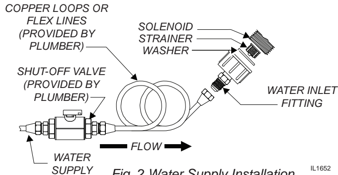
Fig. 2 Water Supply Installation New-style shown
