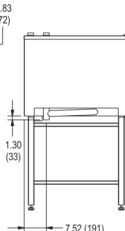
BACK VIEW
