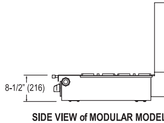
SIDE VIEW of MODULAR MODEL
