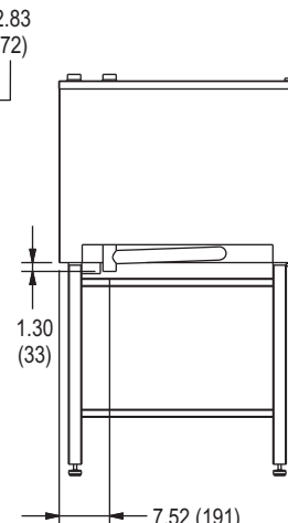
BACK VIEW
