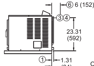
SIDE VIEWS
