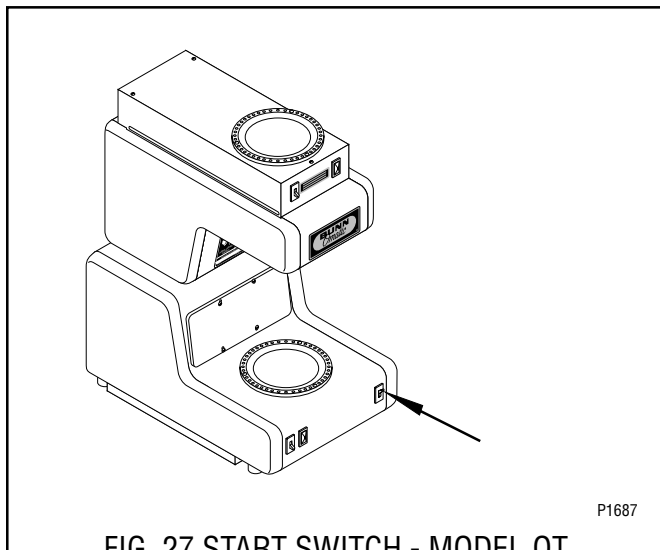
FIG. 27 START SWITCH - MODEL OT
