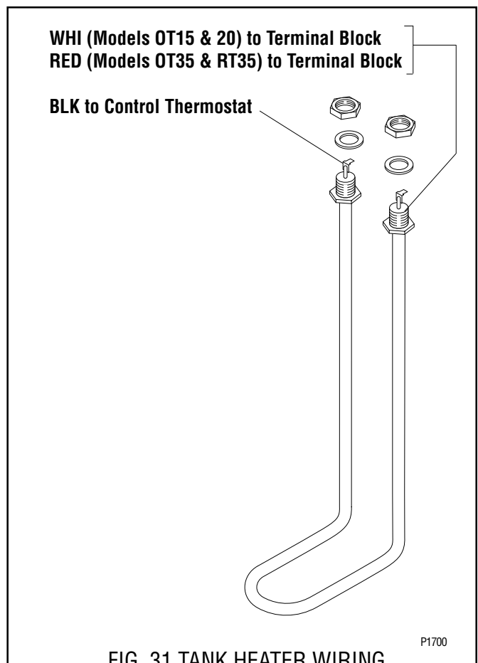
FIG. 31 TANK HEATER WIRING
