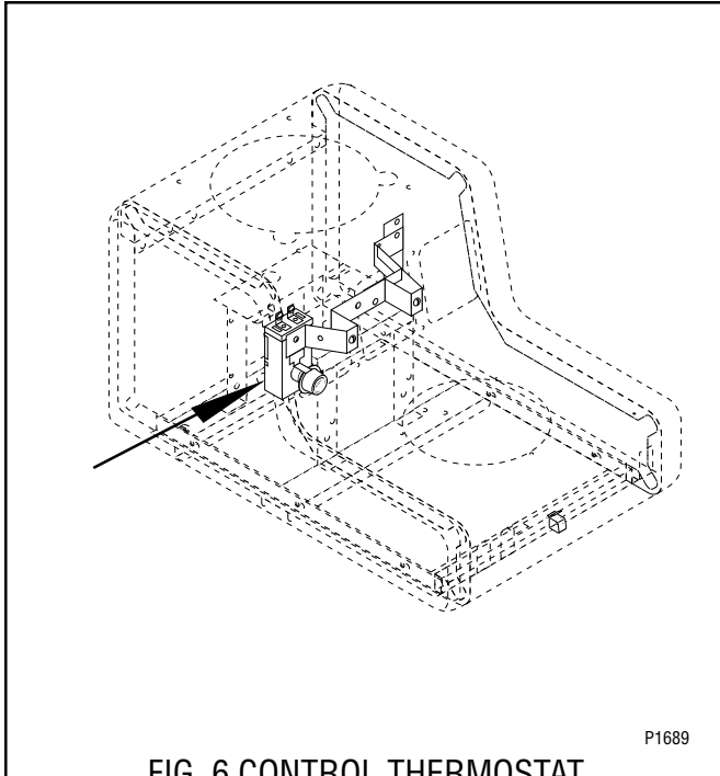
FIG. 6 CONTROL THERMOSTAT
