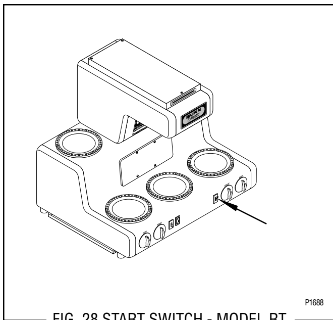
FIG. 28 START SWITCH - MODEL RT
