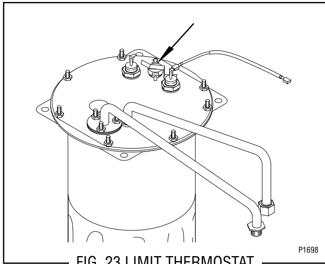
FIG. 23 LIMIT THERMOSTAT
