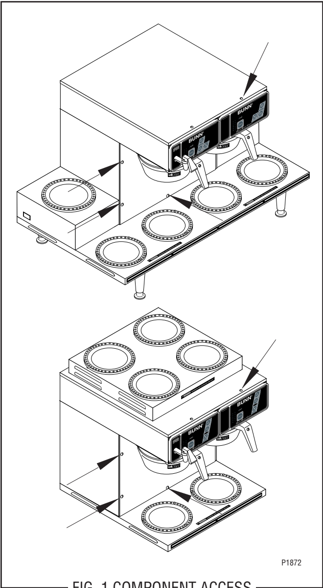
FIG. 1 COMPONENT ACCESS
