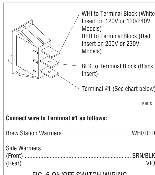
FIG. 6 ON/OFF SWITCH WIRING
