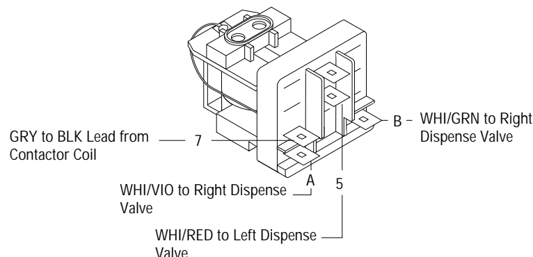
ELECTRONIC CONTROL W/RECOVERY BOOSTER
