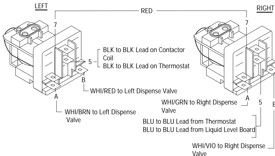
MECHANICAL THERMOSTAT W/RECOVERY BOOSTER
