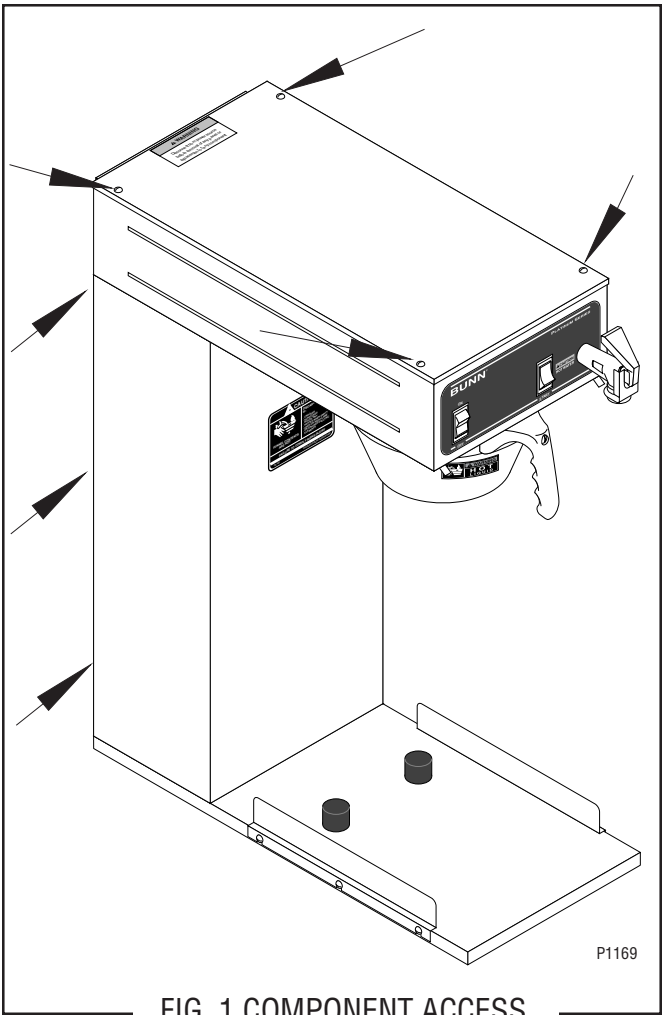
FIG. 1 COMPONENT ACCESS
