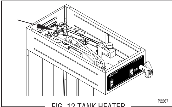
FIG. 12 TANK HEATER
