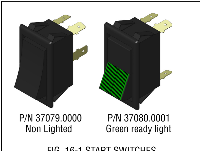
FIG. 16-1 START SWITCHES
