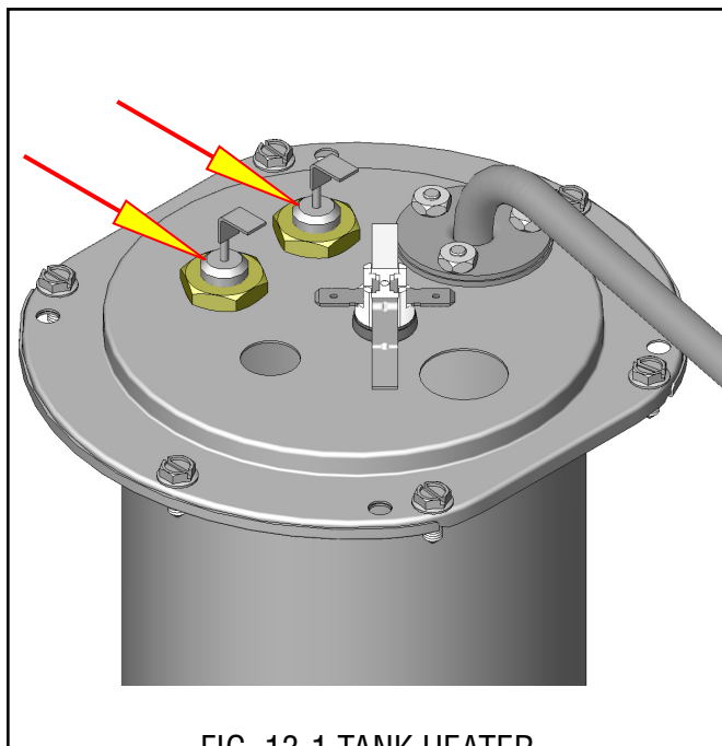
FIG. 13-1 TANK HEATER
