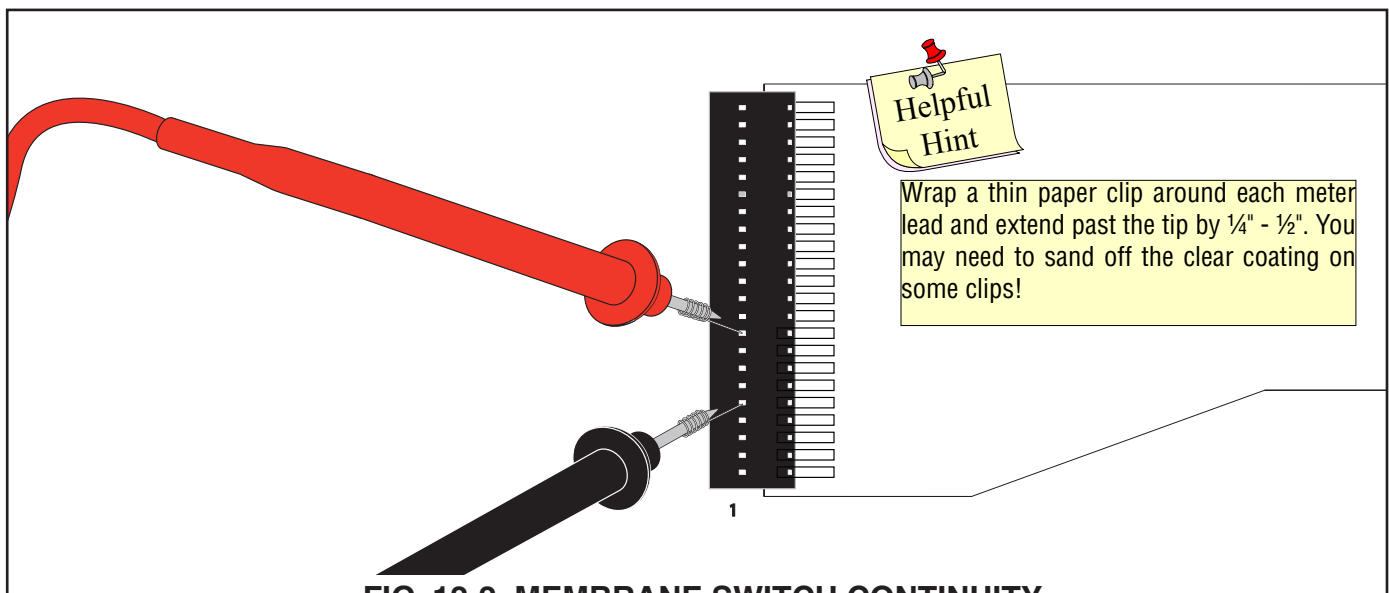
FIG. 12-2 MEMBRANE SWITCH CONTINUITY
