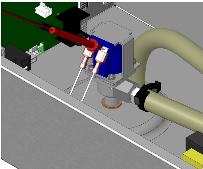
FIG. 14-1 LATE MODEL BREW VALVE
