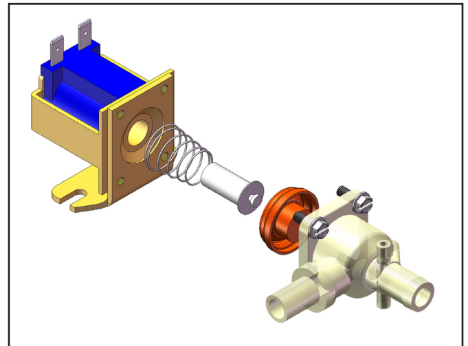
FIG. 13-2 EXPLODED VIEW
