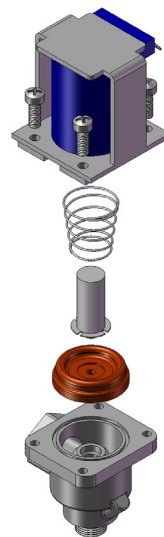
FIG. 14-2 LATE MODEL BREW VALVE
