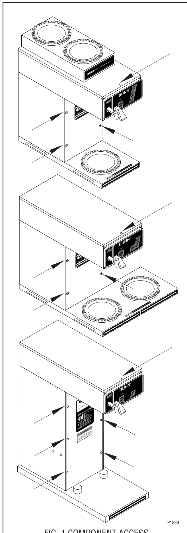
FIG. 1 COMPONENT ACCESS
