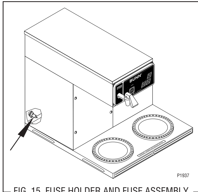
FIG. 15 FUSE HOLDER AND FUSE ASSEMBLY
