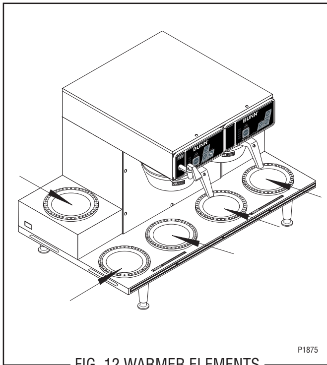
FIG. 12 WARMER ELEMENTS
