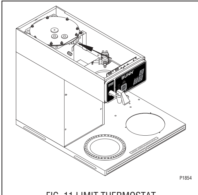
FIG. 11 LIMIT THERMOSTAT
