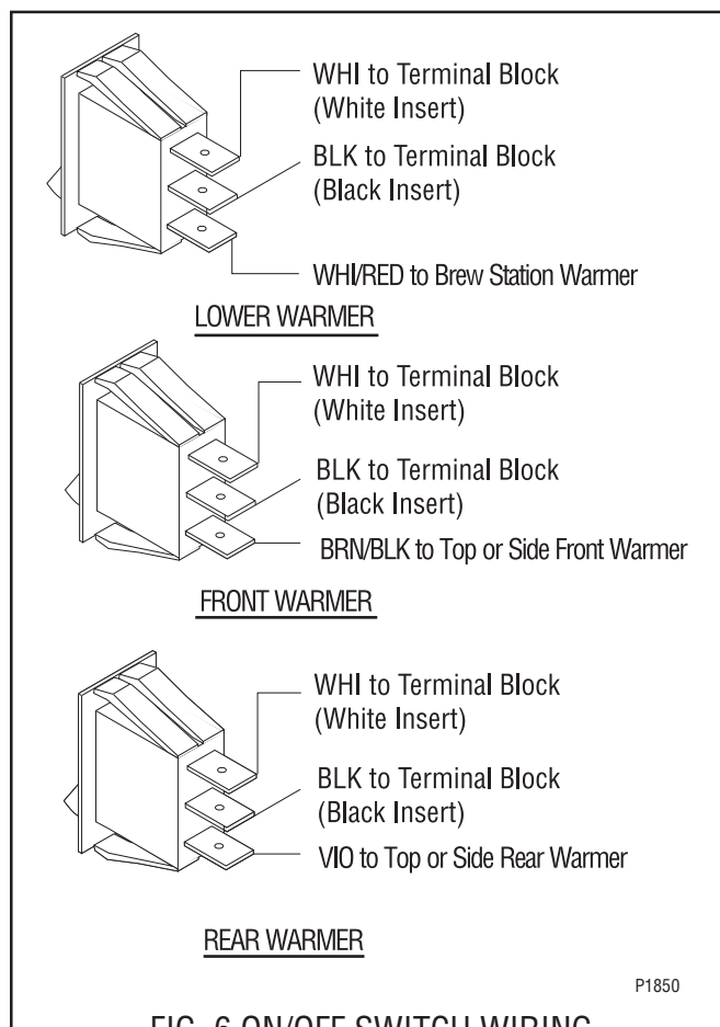
FIG. 6 ON/OFF SWITCH WIRING
