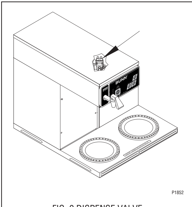
FIG. 9 DISPENSE VALVE
