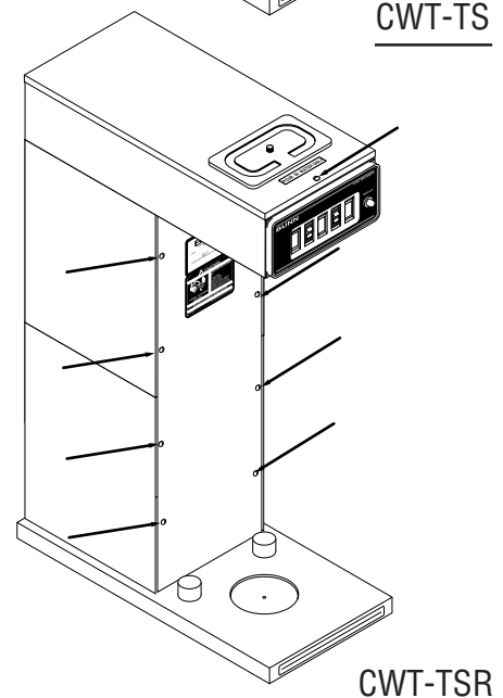
FIG. 1 COMPONENT ACCESS
