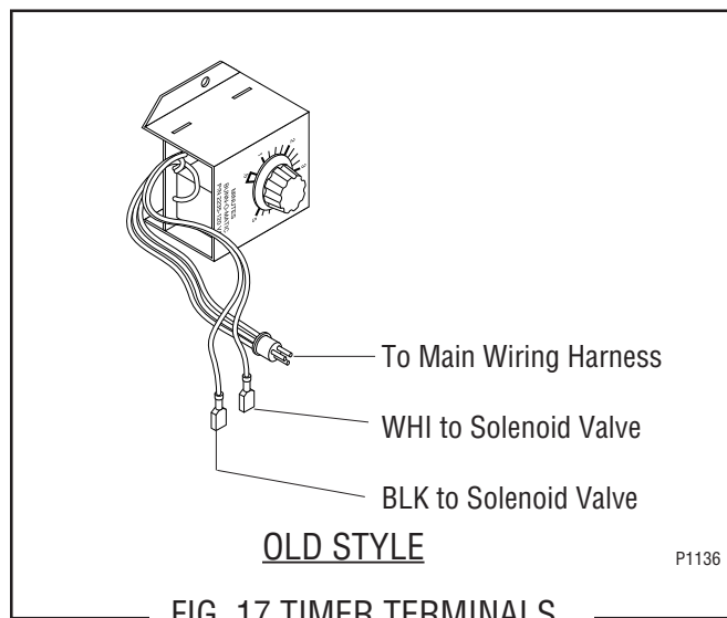
FIG. 17 TIMER TERMINALS
