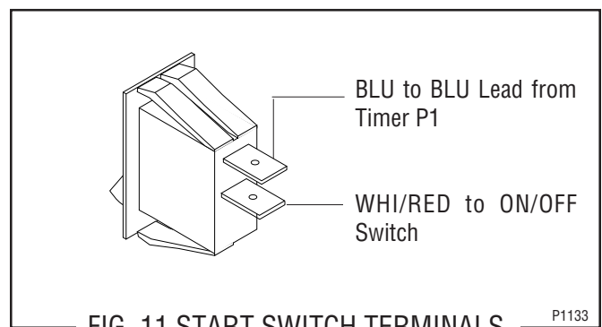
FIG. 11 START SWITCH TERMINALS
