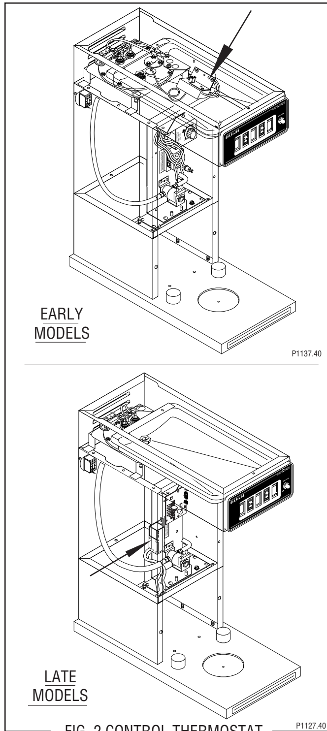
FIG. 2 CONTROL THERMOSTAT
